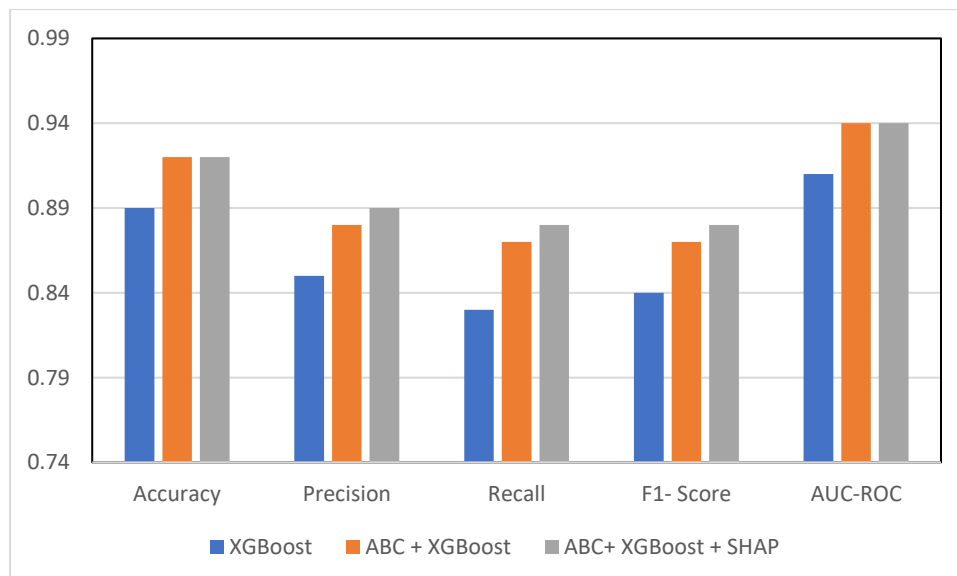
Figure 2: Performance Analysis Chart for Base Methods compared with our proposed method
