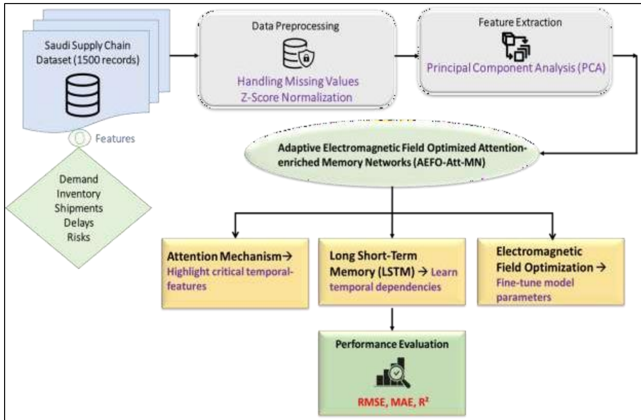
Figure 1. Structural Flow of the Proposed Model
