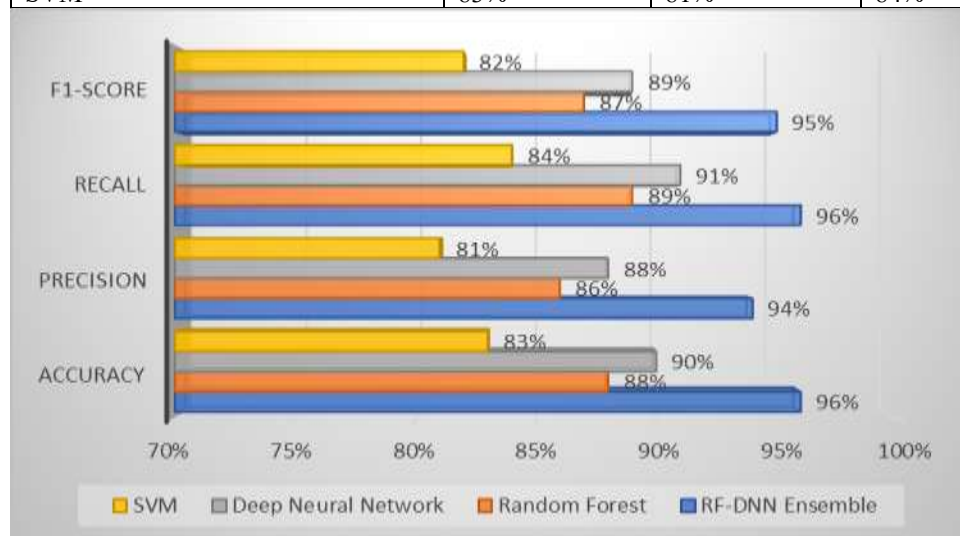
Figure 1: Classification Performance of Different Models
